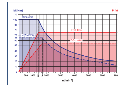
Main spindle / counter spindle motor characteristics
