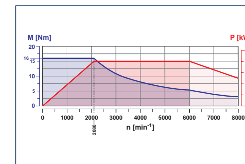
Characteristic for driven tools MT45-HSC tool turret
